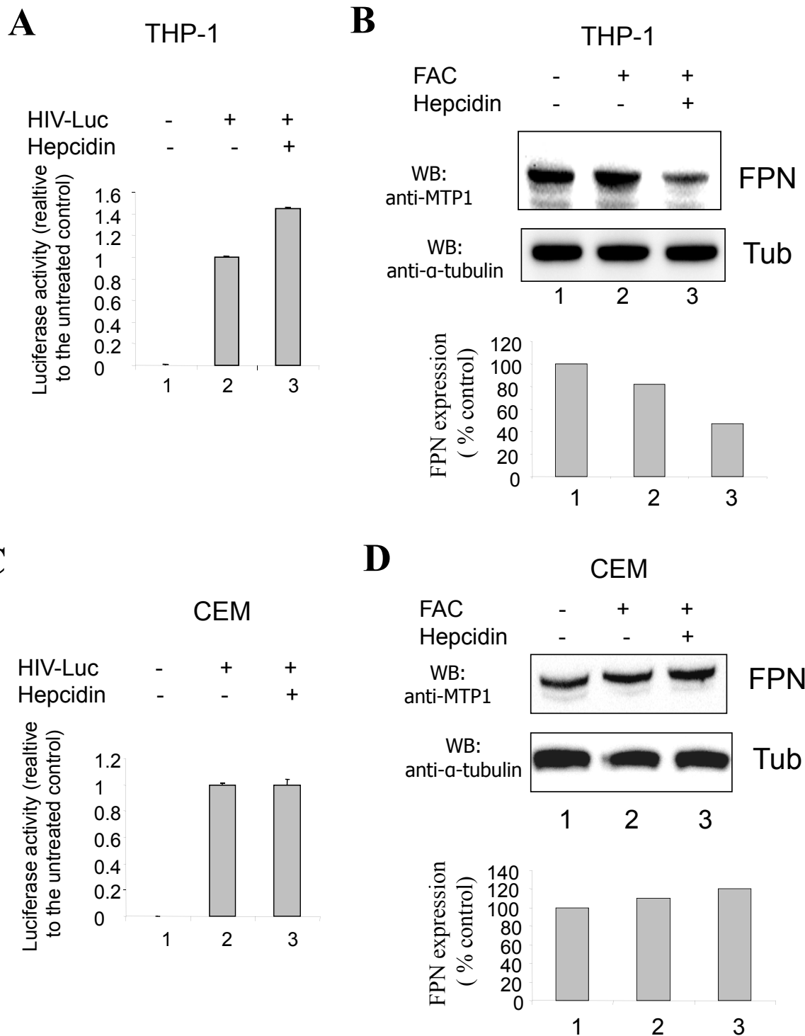
Figure 5 Expression of ferroportin and effect of hepcidin in cultured THP-1 and CEM cells. THP-1 cells (A) or CEM T cells (C) were treated with FAC for 24 hrs and then treated with 100 \mu M ascorbic acid for 2 hours. The cells were then infected with VSVG-pseudotyped HIV-1 Luc virus for 48 hrs (A and C, lanes 2 and 3). Lane 3, the cells were treated with 0.5 \mu M hepcidin for 6 hours. The cells were lysed, using LucLite buffer system and the Luciferase activity was measured using Labsystems Luminoskan and the data normalization to the protein concentration. THP-1 cells (B) or CEM T-cells (D) were treated with FAC for 24 hrs and then with 100 \mu M ascorbic acid for 2 hours (lane 2). The cells were then treated with 0.5 \mu M hepcidin for 6 hours (lane 3). The cell lysates were resolved on 10% SDS-PAGE and immunoblotted with anti-MPT1 antibodies or with anti-tubulin antibodies. Lane 1, untreated control cells.
